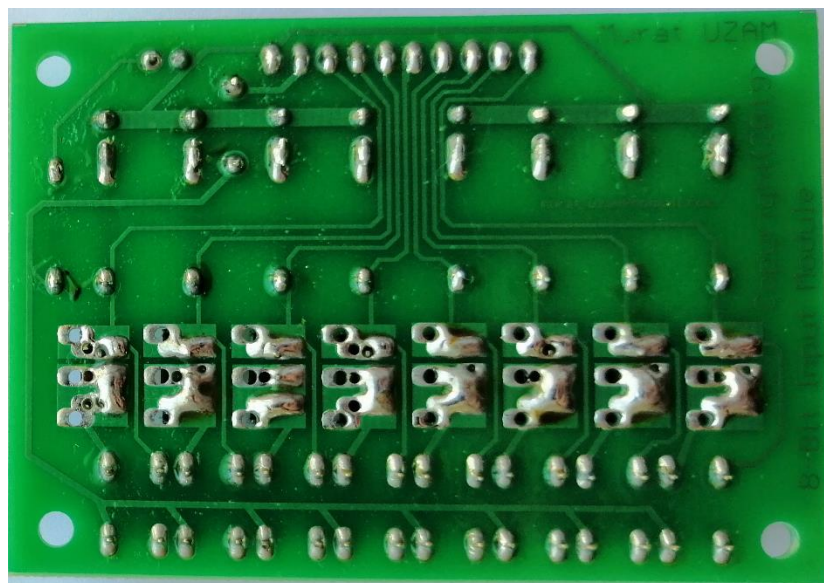
Bottom view (solder side) of the soldered 8-Bit Input Module.
