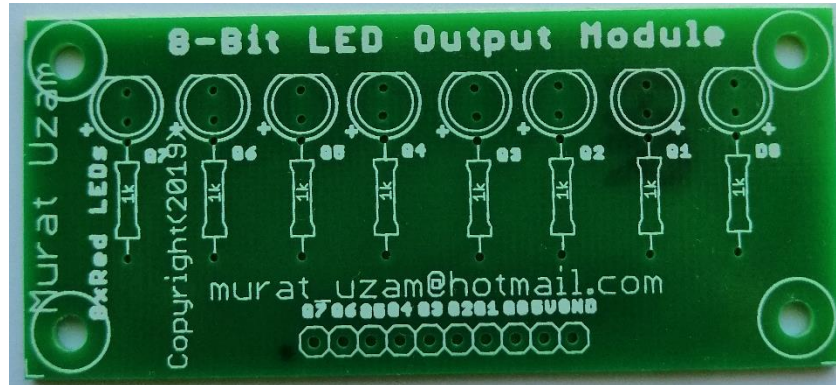
Top view (component side) of the 8-Bit LED Output Module PCB.
