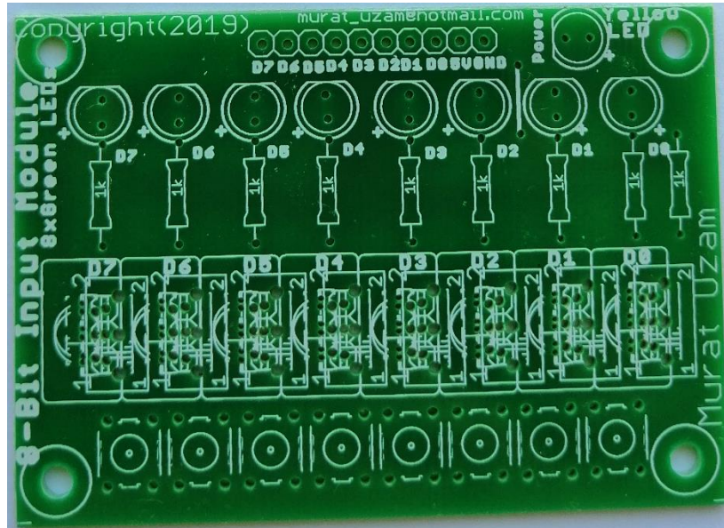
Top view (component side) of the 8-Bit Input Module PCB.
