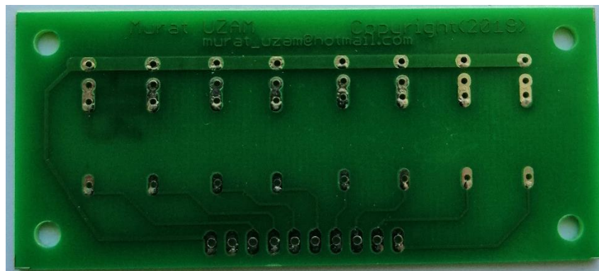
Bottom view (solder side) of the 8-Bit LED Output Module PCB.
