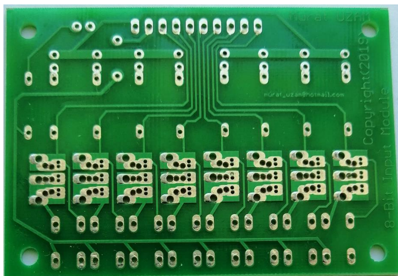
Bottom view (solder side) of the 8-Bit Input Module PCB.
