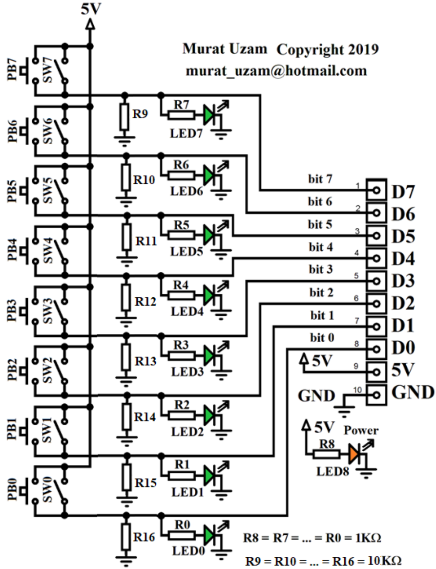
Schematic diagram of the 8-Bit Input Module.
