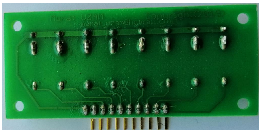
Bottom view (solder side) of the soldered 8-Bit LED Output Module.
