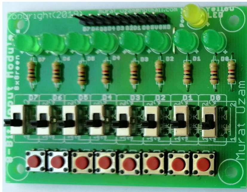
Top view (component side) of the soldered 8-Bit Input Module.
